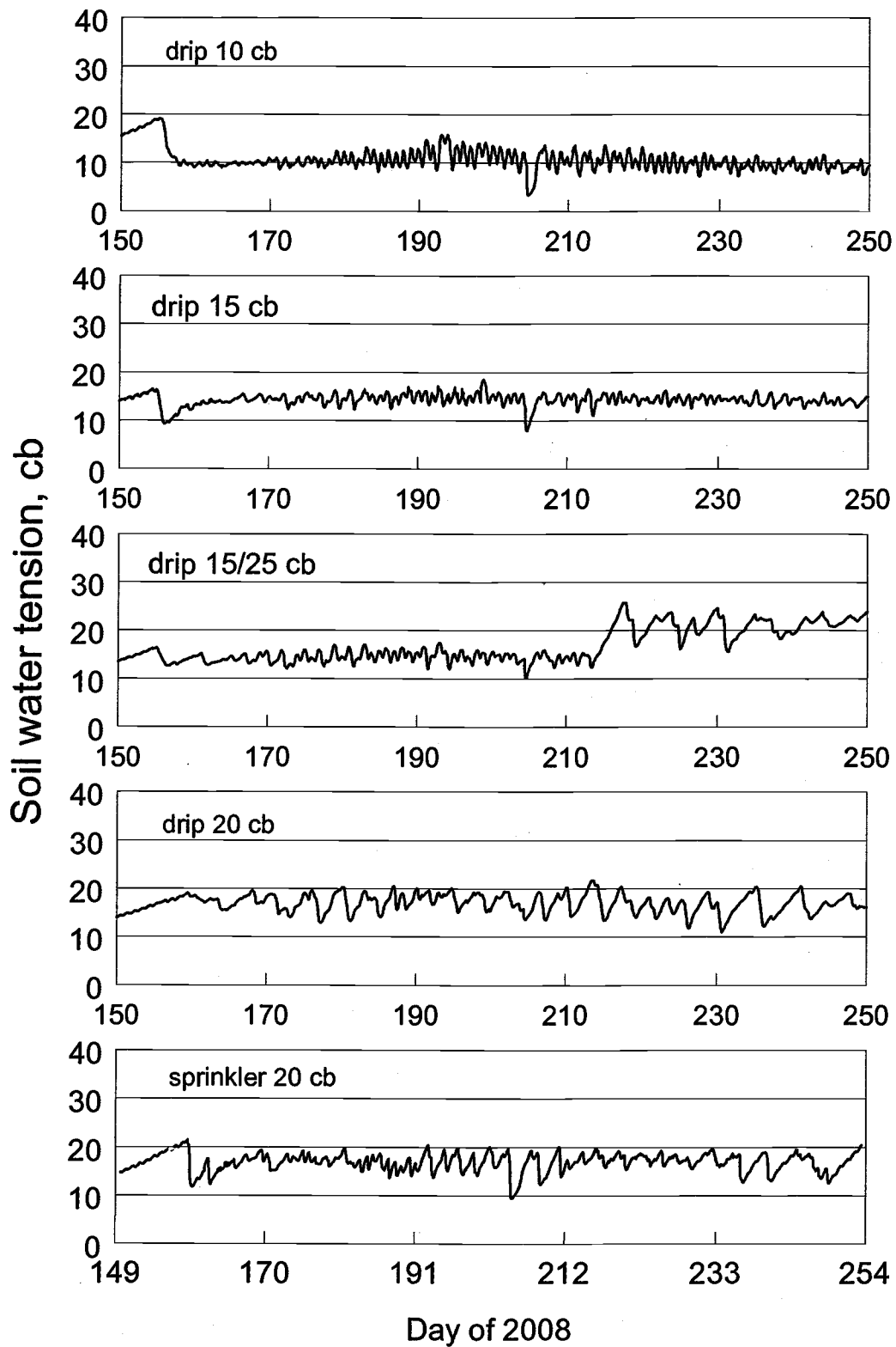
Figure 1a. Soil water tension at 8-inch depth over time for onions submitted to nine irrigation treatments, Malheur Experiment Station, Oregon State University, Ontario, OR, 2008.
