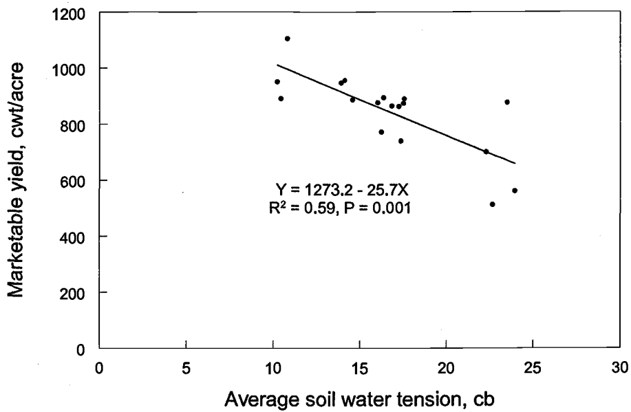
Figure 4. For drip-irrigated onion treatments (averaged over N rate and variety) the average soil water tension was negatively related to marketable yield. Malheur Experiment Station, Oregon State University, Ontario, OR, 2008.
