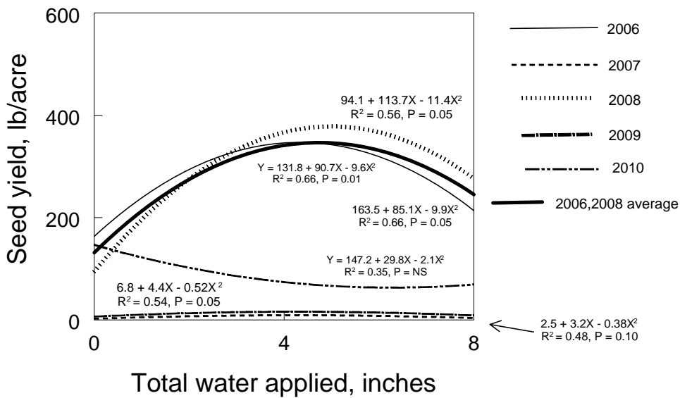
Figure 10. Annual and 2-year average Penstemon speciosus seed yield response to irrigation water, Malheur Experiment Station, Oregon State University, Ontario, OR, 2010.
