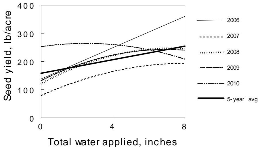
Figure 8. Average annual Eriogonum umbellatum seed yield response to irrigation water applied in 5 years and averaged over 5 years, Malheur Experiment Station, Oregon State University, Ontario, OR, 2010. Regression equations: 2006, Y = 137.9 + 27.8X , R^2 = 0.68 , P = 0.01 ; 2007, Y = 79.6 + 28.3X - 1.75X^2 , R^2 = 0.69 , P = 0.05 ; 2008, Y = 121.3 + 34.6X - 2.4X^2 , R^2 = 0.73 , P = 0.01 ; 2009, Y = 132.3 + 31.9X - 2.3X^2 , R^2 = 0.60 , P = .05 ; 2010, Y = 252.9 + 9.21X - 1.8X^2 , R^2 = 0.08 , P = \text{NS} ; 5-year average, Y = 158.3 + 12X , R^2 = 0.77 , P = 0.001 .
