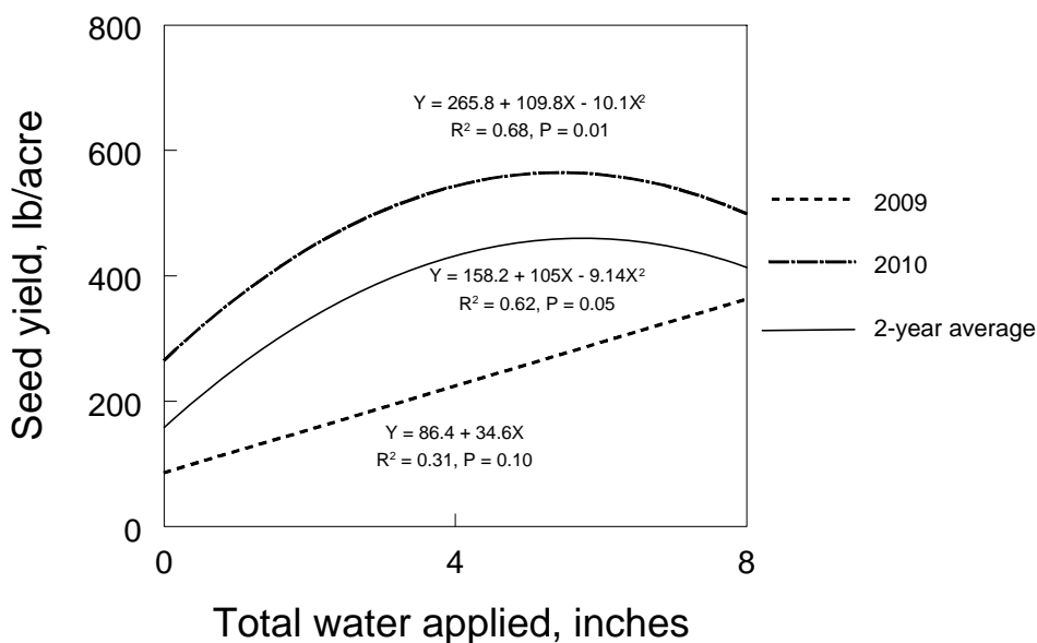
Figure 13. Annual and 2-year average Lomatium dissectum seed yield response to irrigation water, Malheur Experiment Station, Oregon State University, Ontario, OR, 2010.
