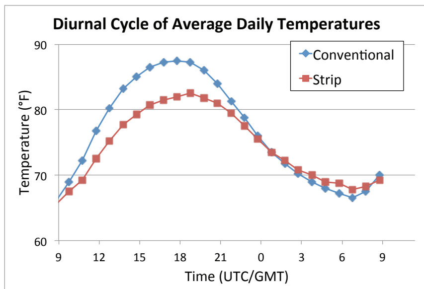
Figure 3. Average daily soil temperatures at 4-inch depth under conventional and strip tillage for a typical day.
