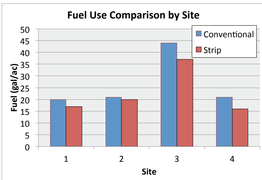
Figure 2. The fuel cost associated with conventional tillage and strip tillage at each of four sites in 2011. Strip tillage required less fuel than conventional tillage at all four sites. However, the fuel costs across sites were variable. The fuel consumptions in Figure 2 are in the same order as the 2011 crops listed in Table 1.
